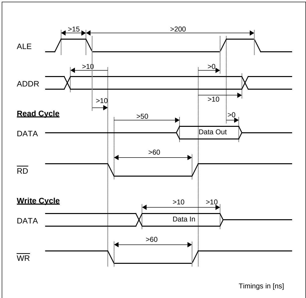
Figure 3-7 Asynchronous Flash Access Cycle in External Host Mode
