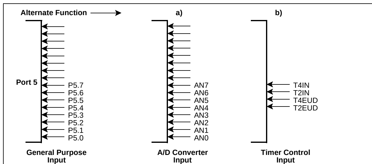
Figure 7-16 Port 5 IO and Alternate Functions
