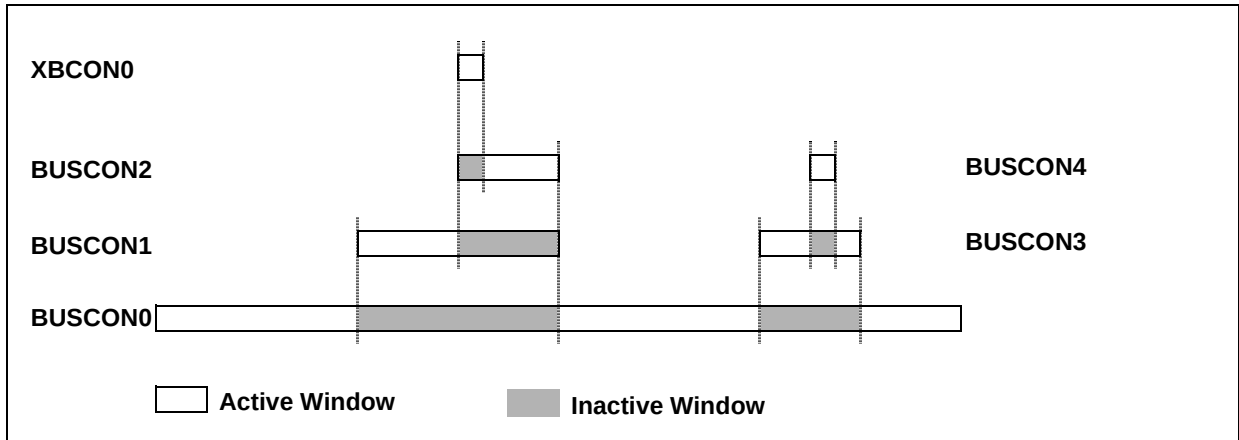
Figure 9-10 Address Window Arbitration
