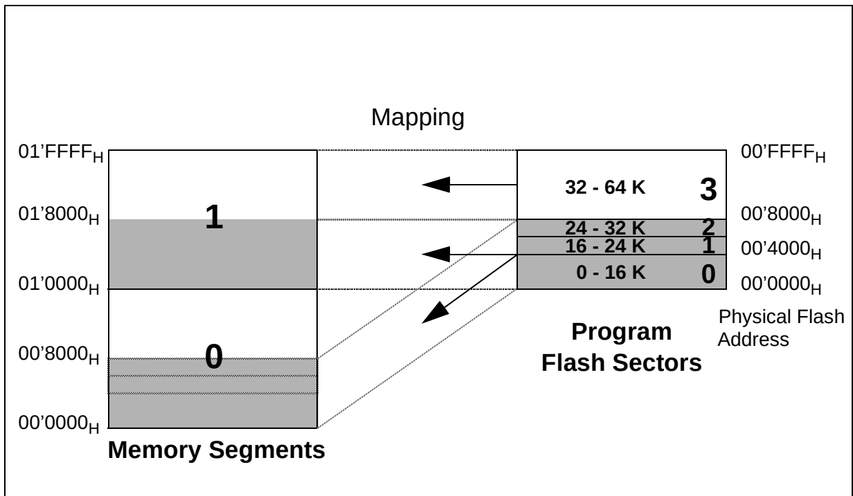
Figure 3-5 Mapping of the On-chip Flash Module Sectors
