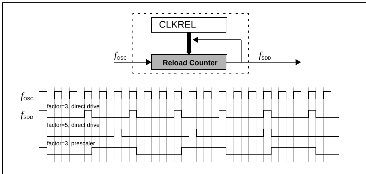
Figure 21-3 Slow Down Divider Operation
