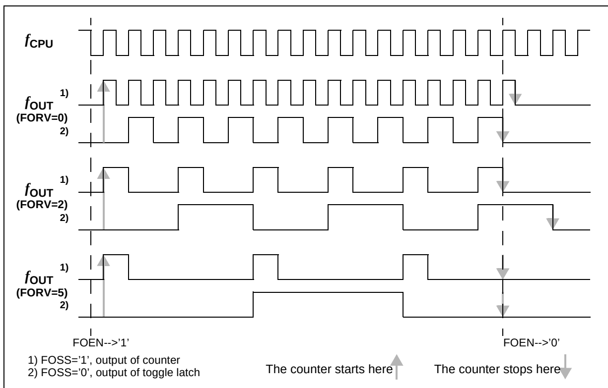
Figure 21-8 Signal Waveforms
